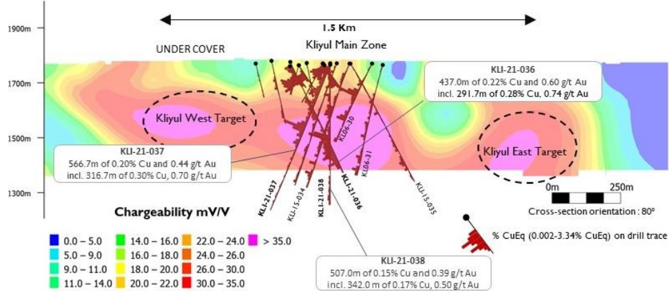
Cross Section of KMZ, Kliyul West and Kliyul East Targets on IP Chargeability – 300 m clipping
